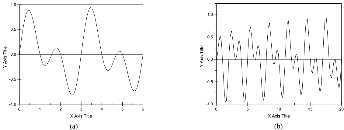
Fig.1 Output voltage waveforms of (a) B and (b) H sensors
